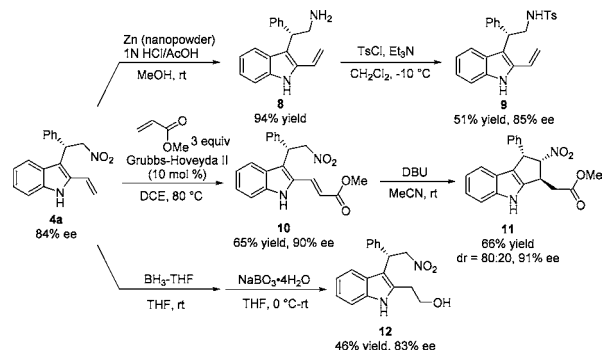
Scheme 3. Transformations of Chiral 2-Vinylindole 4a
