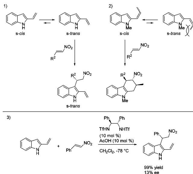
Scheme 4. Reaction Pathway for (1) Friedel–Crafts Reaction and (2) [4 + 2]-Cycloaddition
